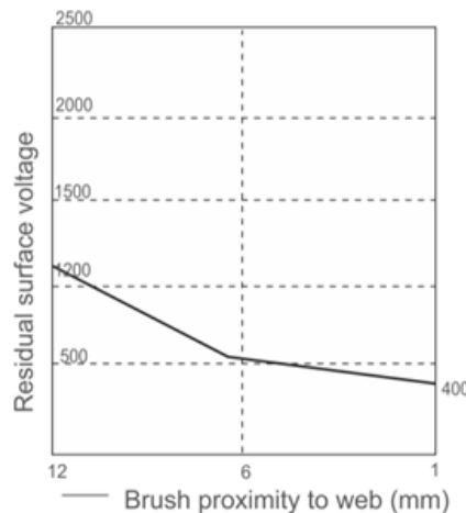
Effectiveness of Valstat passive brush at a web speed of 325 mpm and an initial surface voltage of 10 kV
